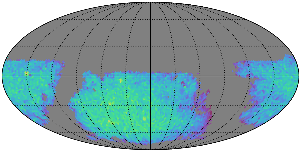
early_u_fpextra4.0_v3.4_10yrs gi: LVDwarfs
