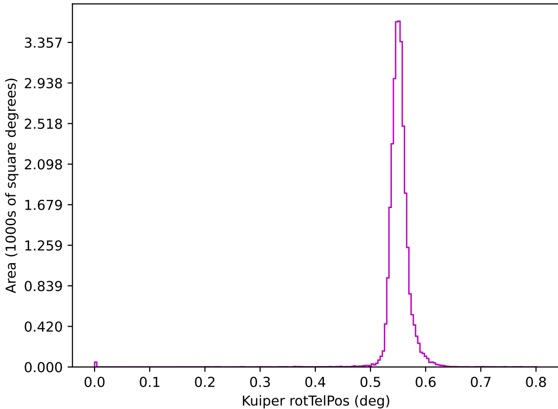
early_u_fpextra4.0_v3.4_10yrs z: Kuiper rotTelPos
