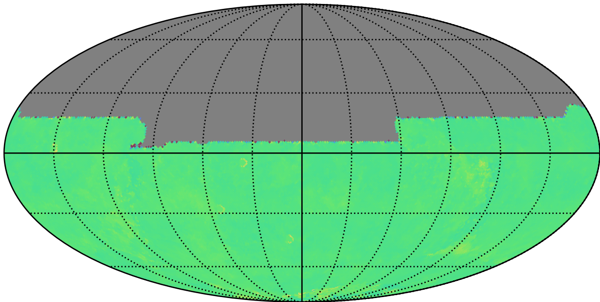
early_u_fpextra4.0_v3.4_10yrs y: Kuiper rotTelPos
