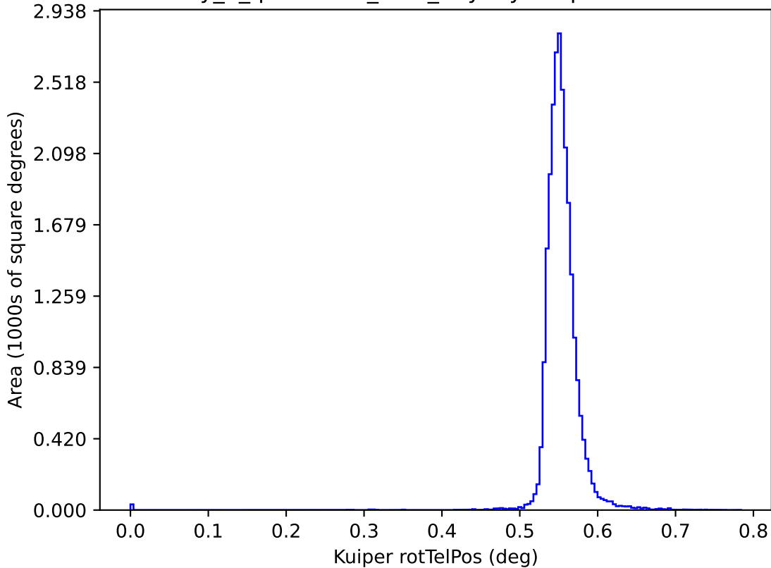
early_u_fpextra4.0_v3.4_10yrs y: Kuiper rotTelPos
