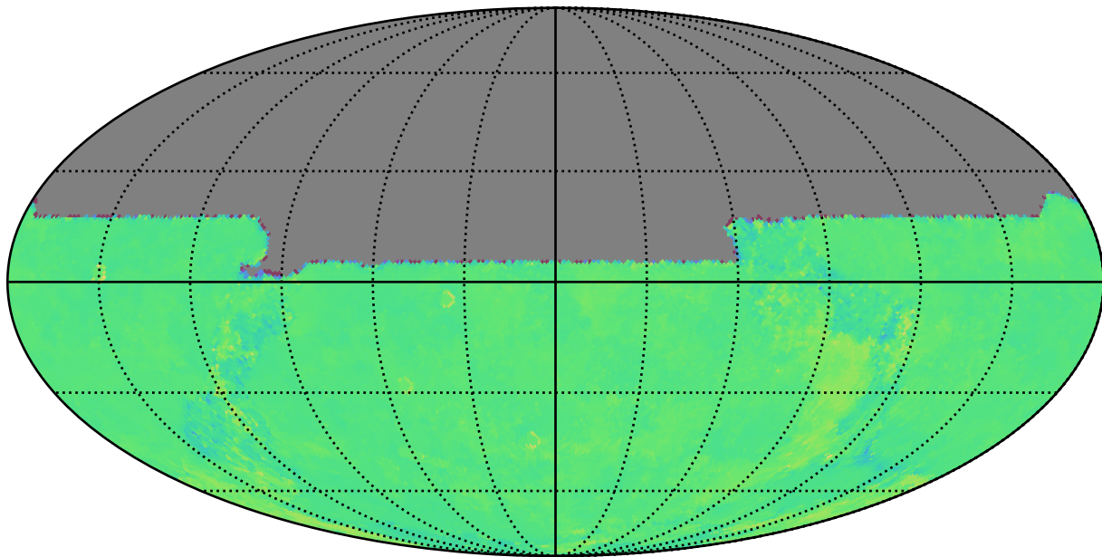
early_u_fpextra4.0_v3.4_10yrs u: Kuiper rotTelPos
