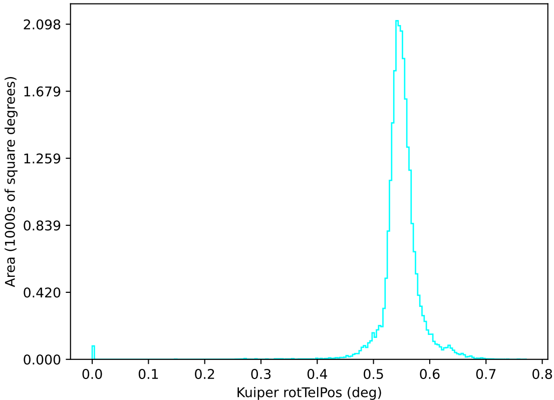
early_u_fpextra4.0_v3.4_10yrs u: Kuiper rotTelPos
