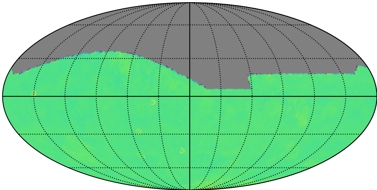
early_u_fpextra4.0_v3.4_10yrs r: Kuiper rotTelPos
