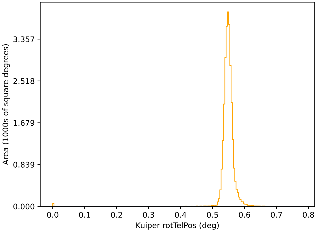
early_u_fpextra4.0_v3.4_10yrs r: Kuiper rotTelPos
