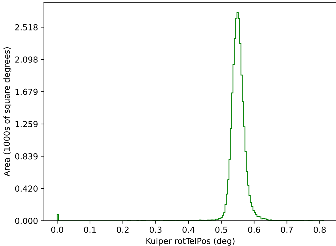
early_u_fpextra4.0_v3.4_10yrs g: Kuiper rotTelPos
