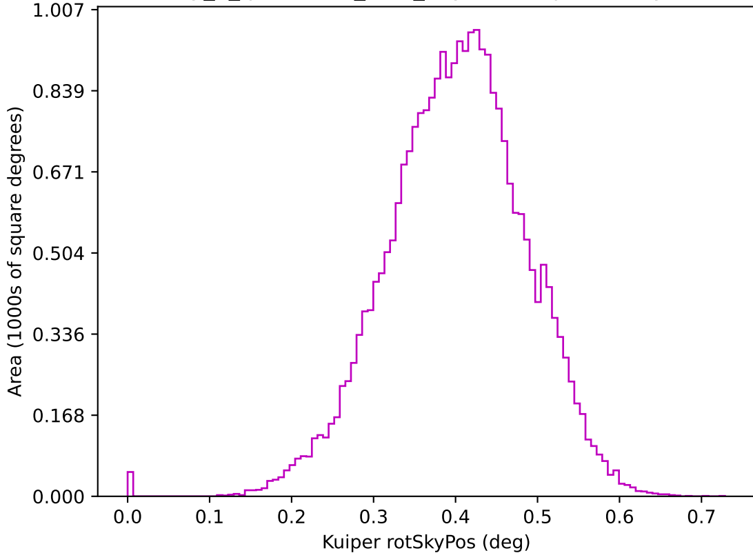
early_u_fpextra4.0_v3.4_10yrs z: Kuiper rotSkyPos
