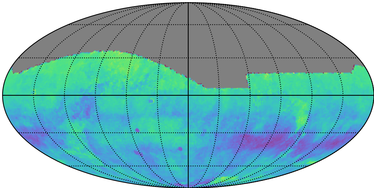
early_u_fpextra4.0_v3.4_10yrs r: Kuiper rotSkyPos
