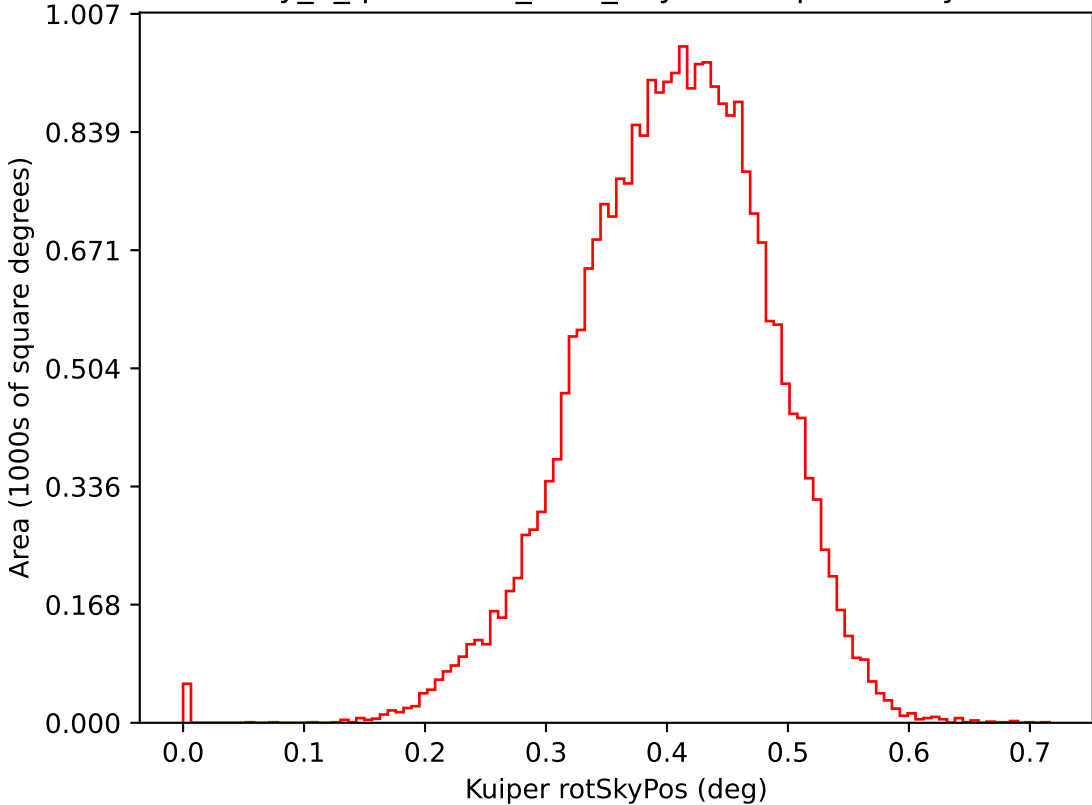
early_u_fpextra4.0_v3.4_10yrs i: Kuiper rotSkyPos
