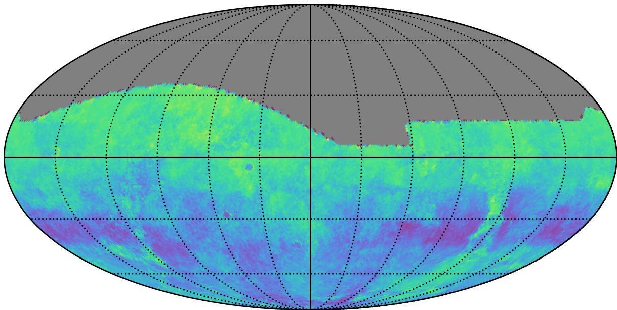
early_u_fpextra4.0_v3.4_10yrs g: Kuiper rotSkyPos
