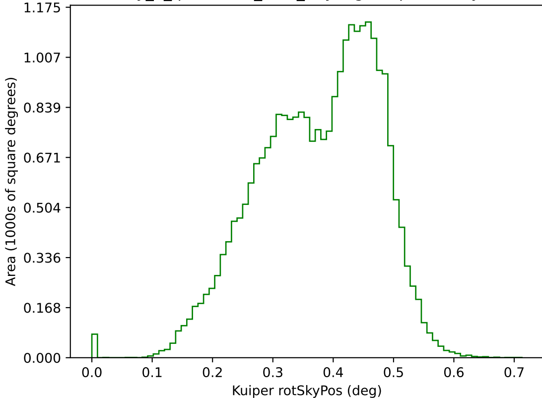
early_u_fpextra4.0_v3.4_10yrs g: Kuiper rotSkyPos
