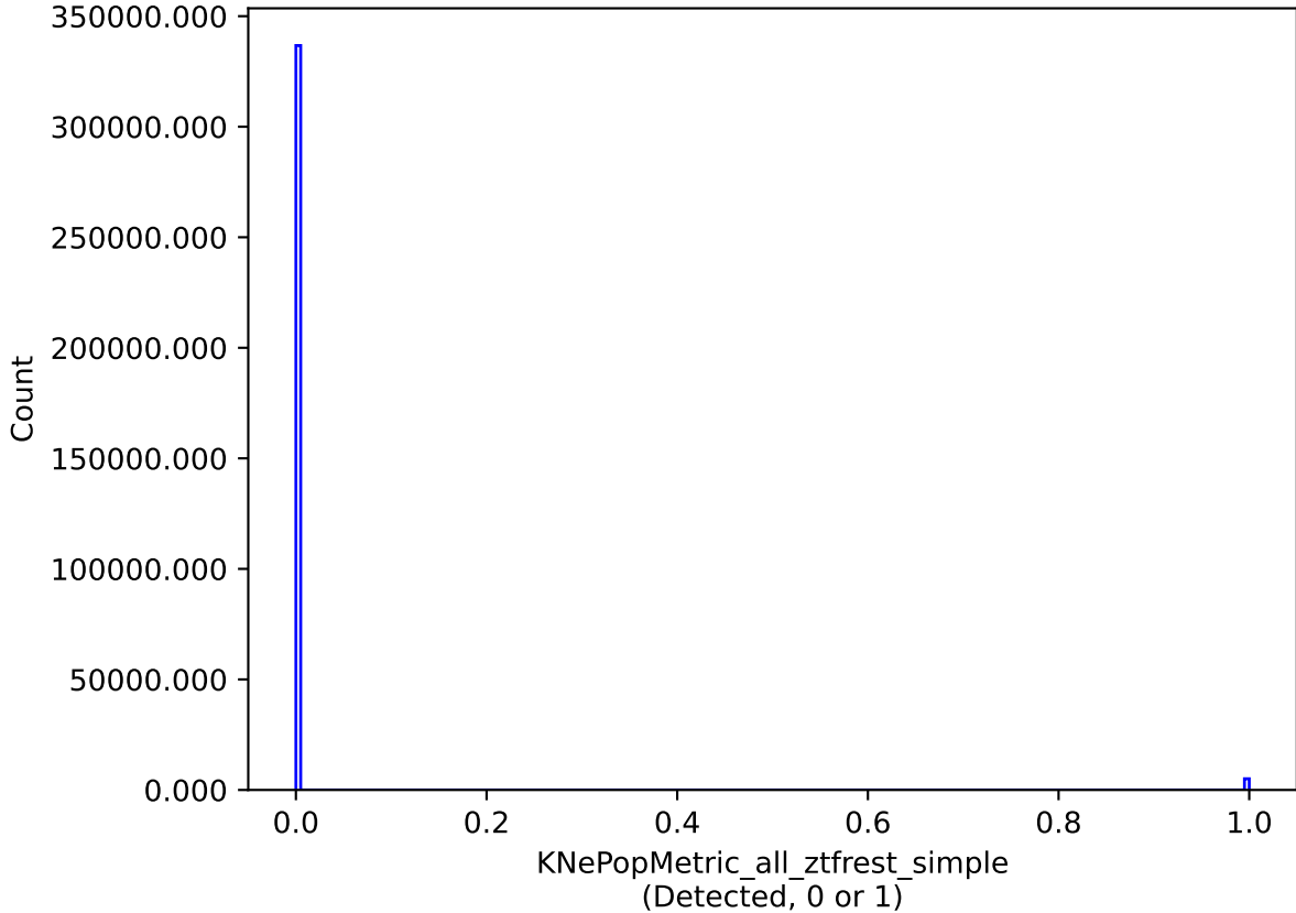
early_u_fpextra4.0_v3.4_10yrs all models: KNePopMetric_all_ztfrest_simple
