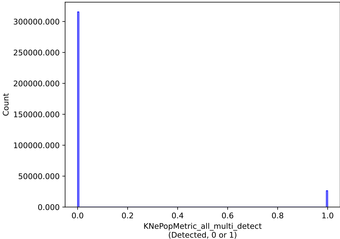
early_u_fpextra4.0_v3.4_10yrs all models: KNePopMetric_all_multi_detect
