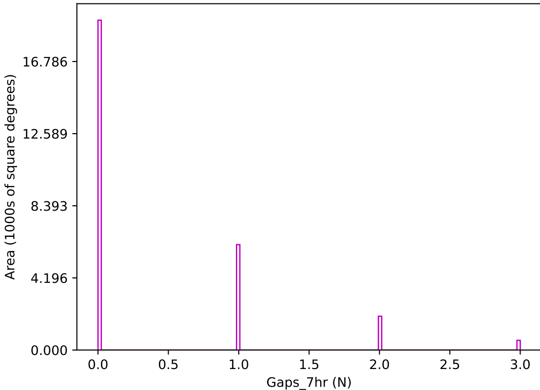
early_u_fpextra4.0_v3.4_10yrs z band: Gaps_7hr
