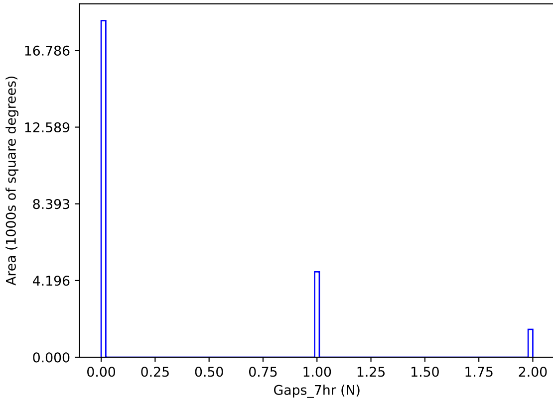
early_u_fpextra4.0_v3.4_10yrs y band: Gaps_7hr
