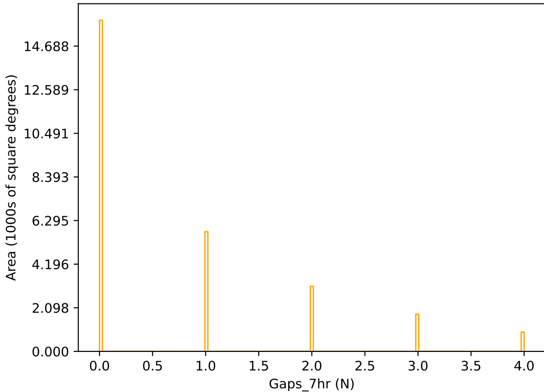
early_u_fpextra4.0_v3.4_10yrs r band: Gaps_7hr
