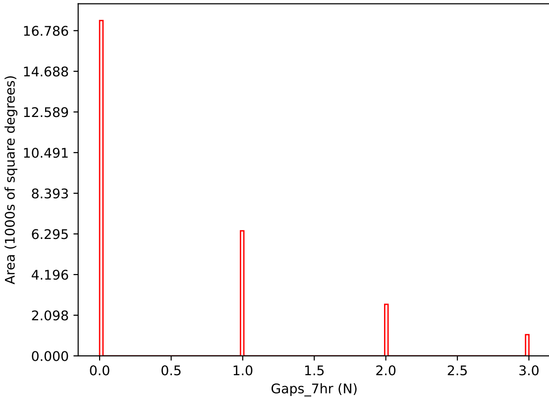
early_u_fpextra4.0_v3.4_10yrs i band: Gaps_7hr
