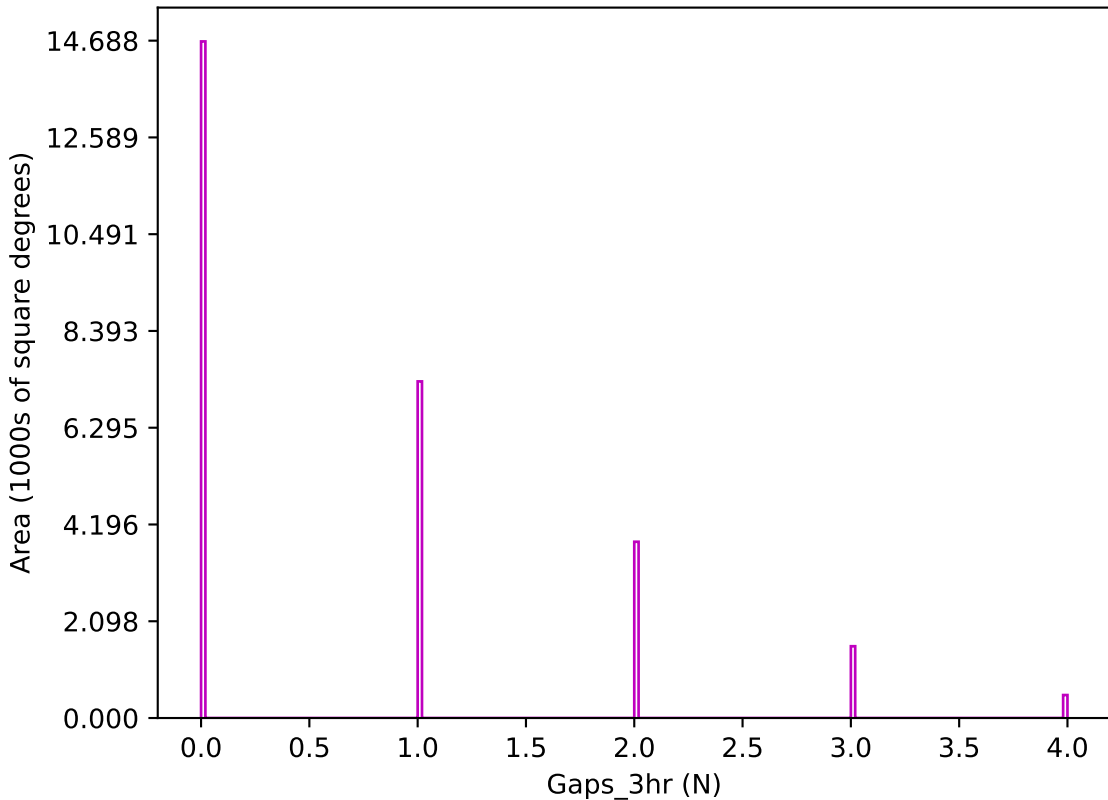
early_u_fpextra4.0_v3.4_10yrs z band: Gaps_3hr
