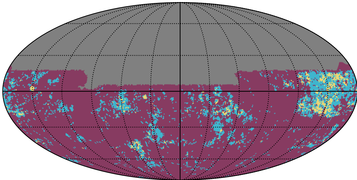
early_u_fpextra4.0_v3.4_10yrs u band: Gaps_3hr
