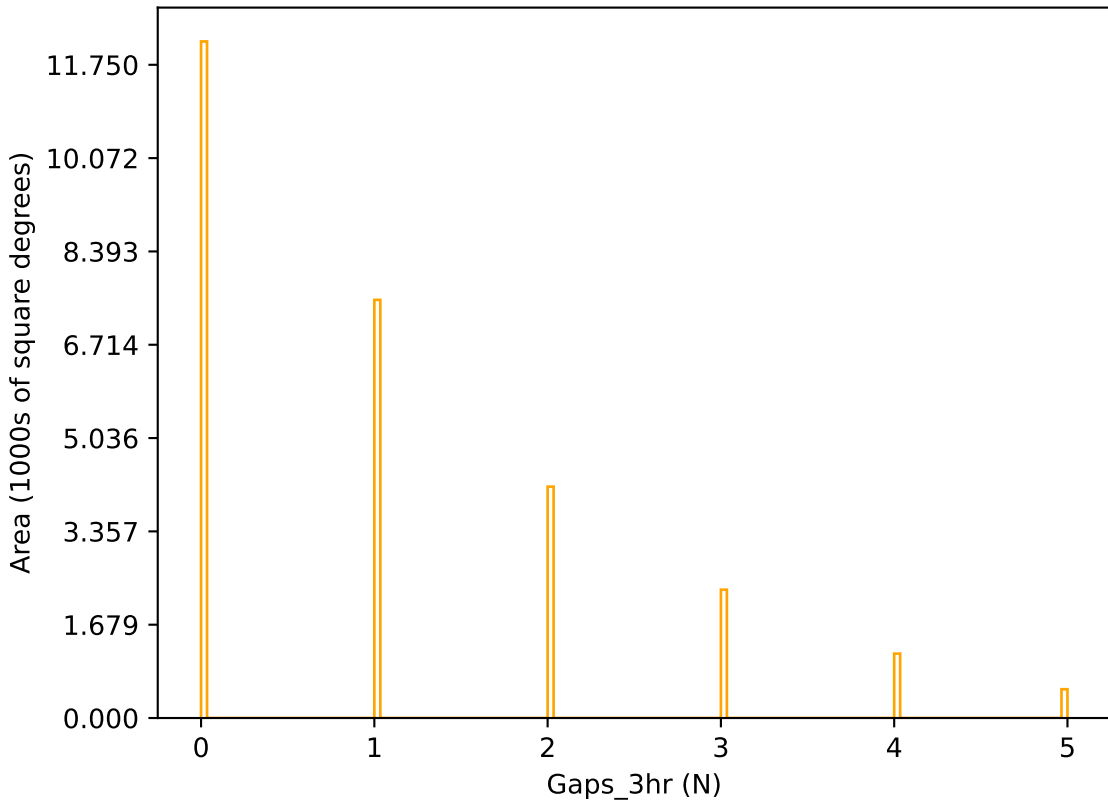
early_u_fpextra4.0_v3.4_10yrs r band: Gaps_3hr
