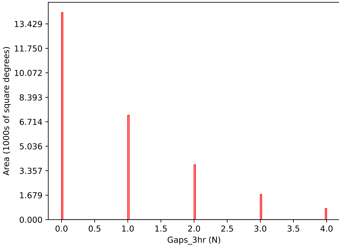
early_u_fpextra4.0_v3.4_10yrs i band: Gaps_3hr
