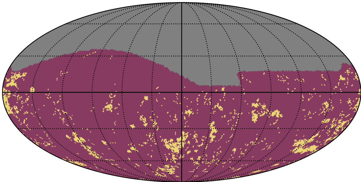
early_u_fpextra4.0_v3.4_10yrs g band: Gaps_3hr
