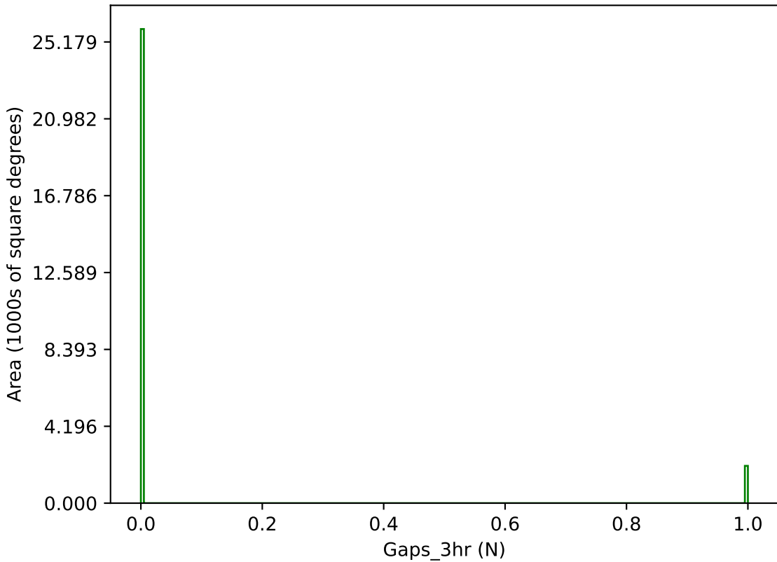
early_u_fpextra4.0_v3.4_10yrs g band: Gaps_3hr
