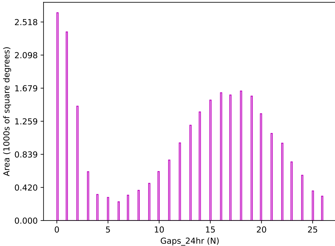
early_u_fpextra4.0_v3.4_10yrs z band: Gaps_24hr
