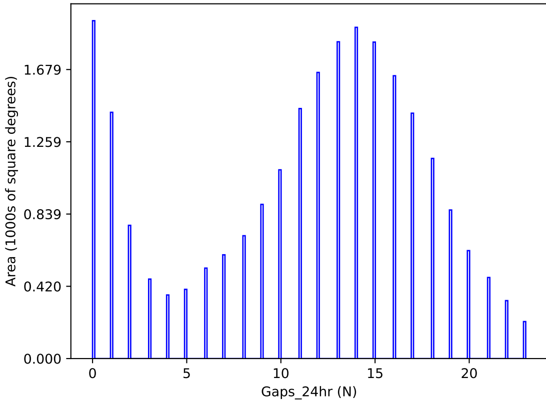
early_u_fpextra4.0_v3.4_10yrs y band: Gaps_24hr
