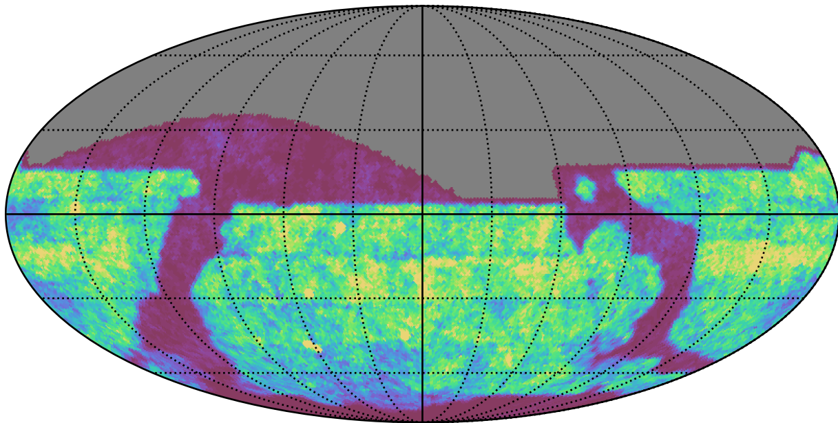
early_u_fpextra4.0_v3.4_10yrs r band: Gaps_24hr
