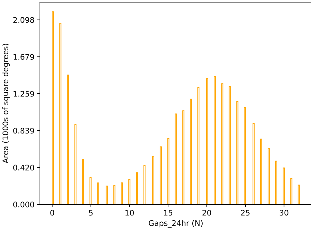
early_u_fpextra4.0_v3.4_10yrs r band: Gaps_24hr
