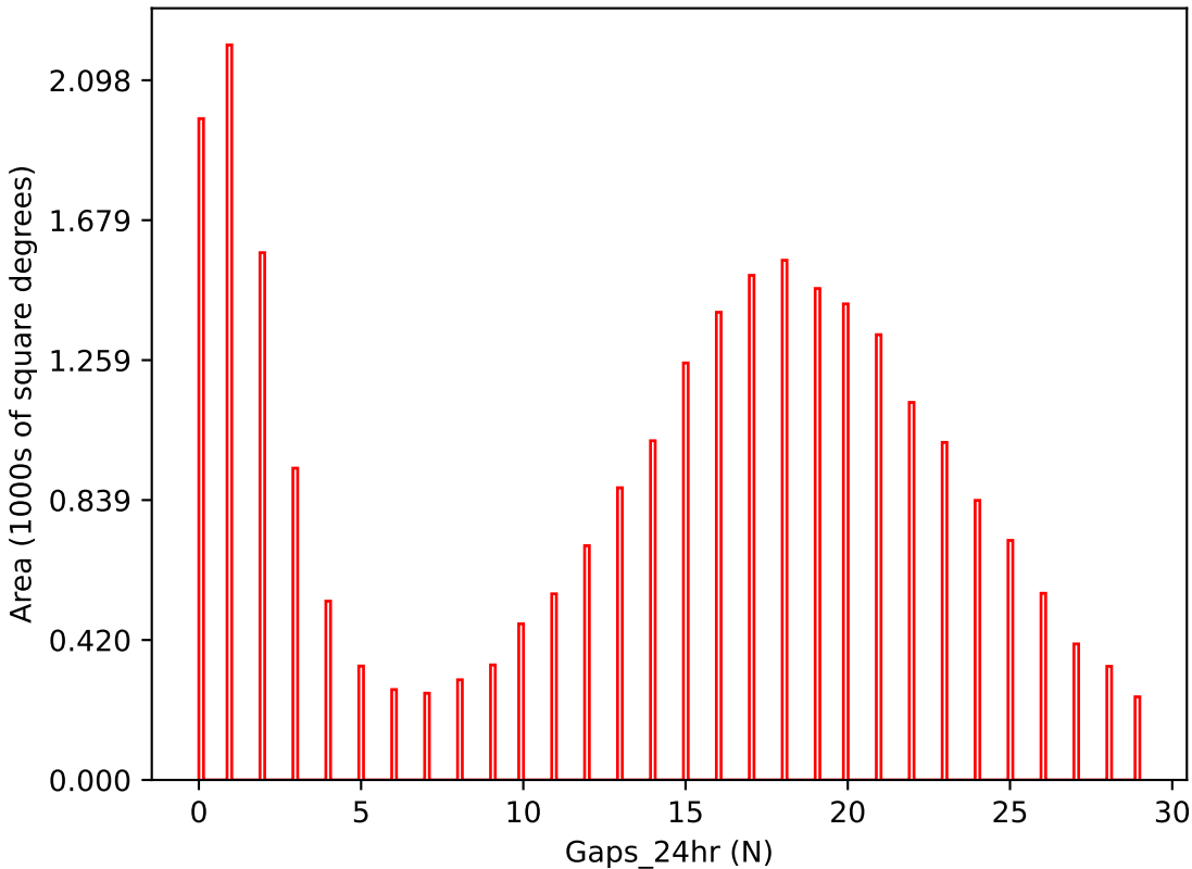
early_u_fpextra4.0_v3.4_10yrs i band: Gaps_24hr
