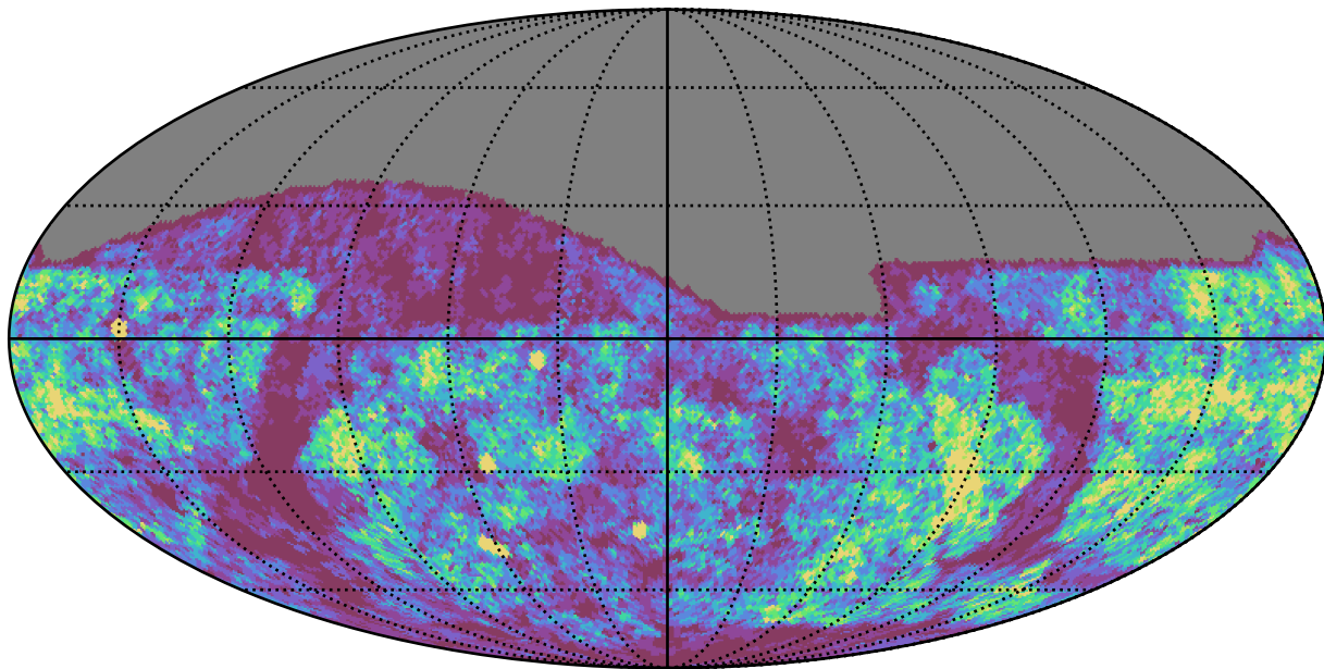
early_u_fpextra4.0_v3.4_10yrs g band: Gaps_24hr
