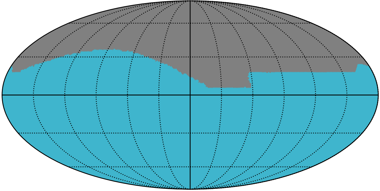
early_u_fpextra4.0_v3.4_10yrs : GalplaneFootprintMetric_xray_binaries_map_Tau_2_0
