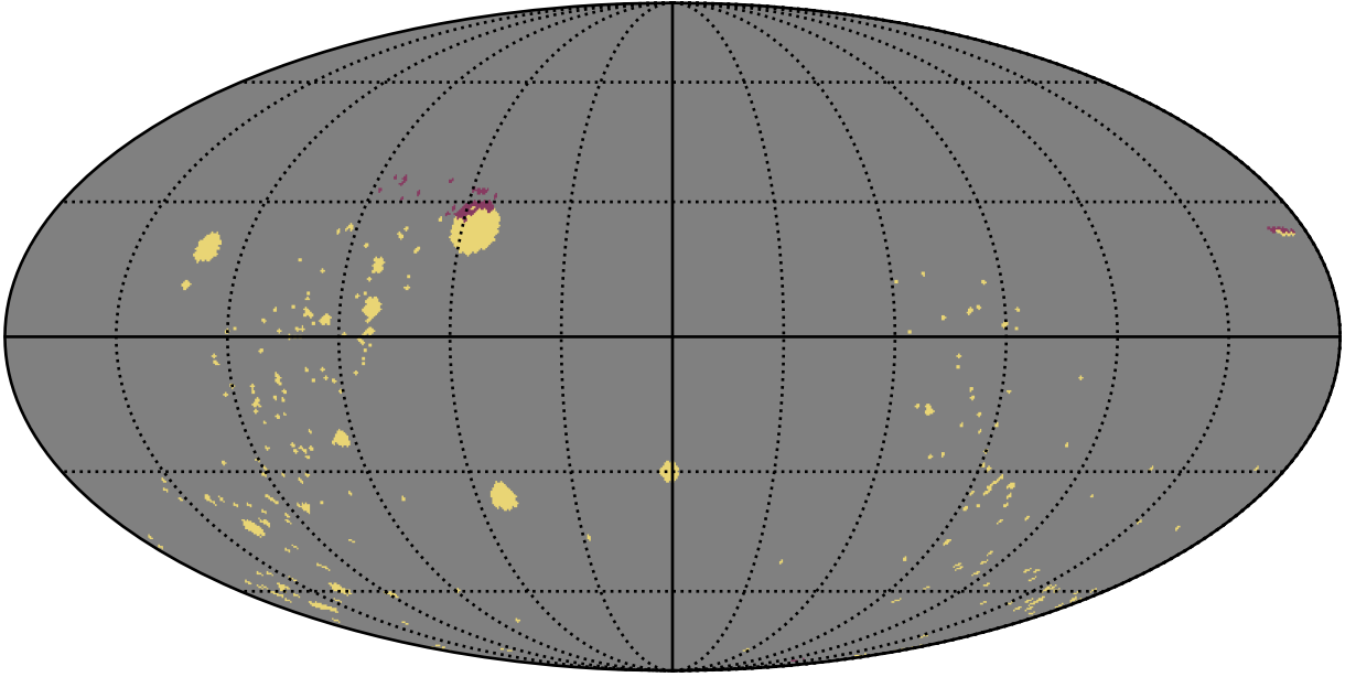
early_u_fpextra4.0_v3.4_10yrs : GalplaneFootprintMetric_open_clusters_map_Tau_73_0
