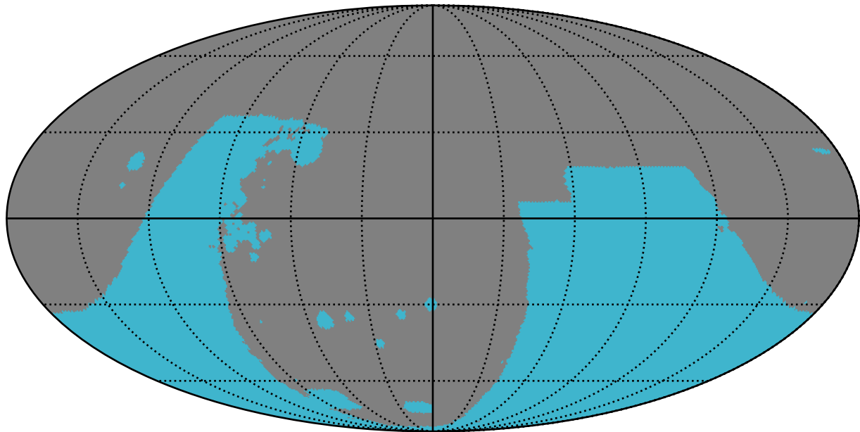
early_u_fpextra4.0_v3.4_10yrs : GalplaneFootprintMetric_combined_map_Tau_2_0
