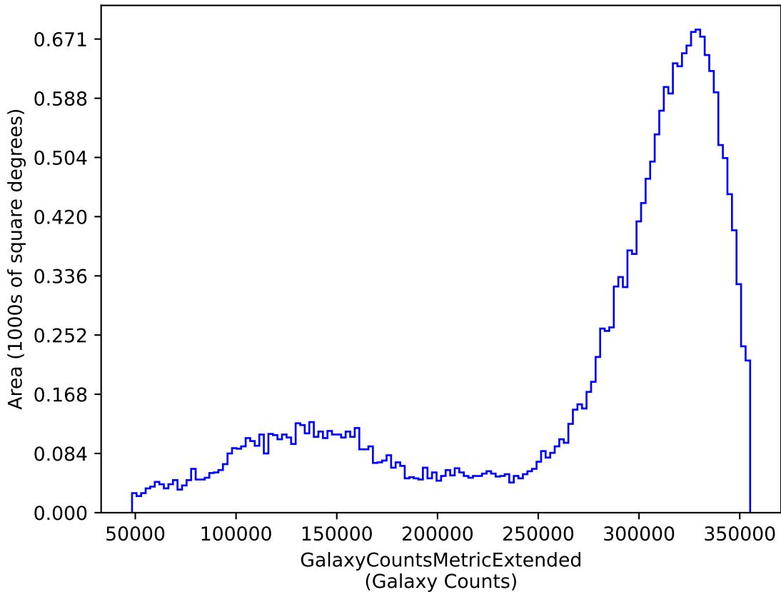
early_u_fpextra4.0_v3.4_10yrs y: GalaxyCountsMetricExtended
