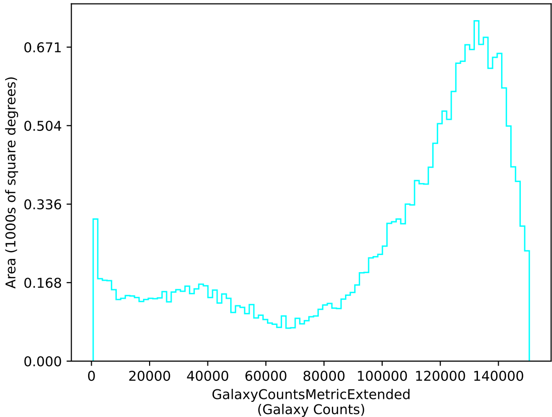
early_u_fpextra4.0_v3.4_10yrs u: GalaxyCountsMetricExtended
