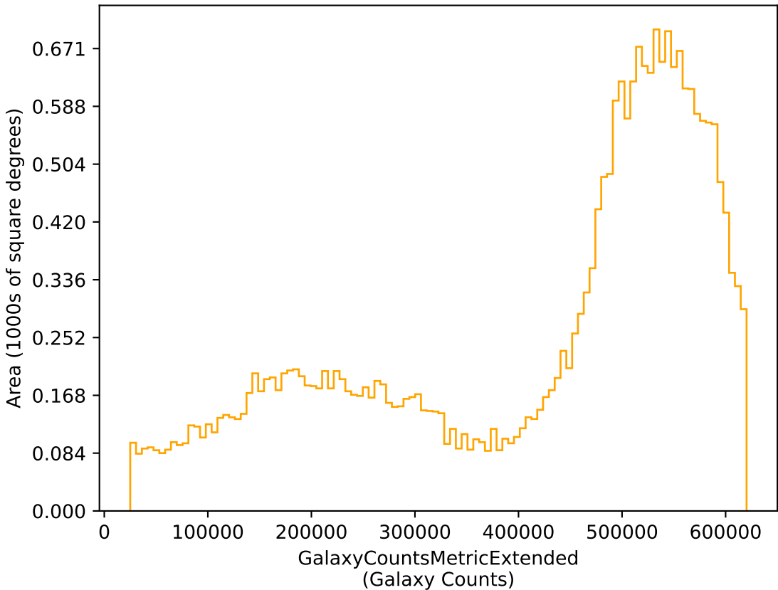
early_u_fpextra4.0_v3.4_10yrs r: GalaxyCountsMetricExtended
