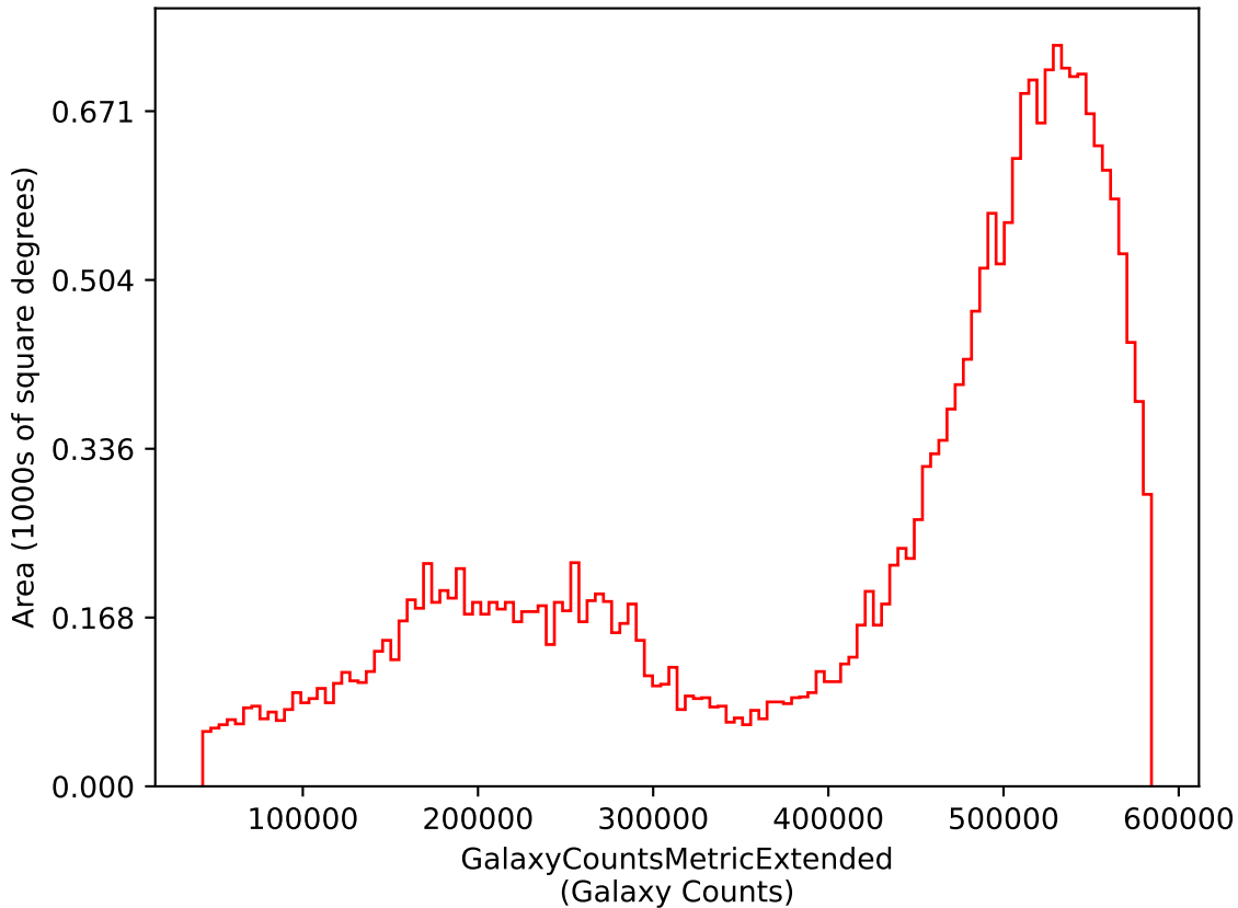
early_u_fpextra4.0_v3.4_10yrs i: GalaxyCountsMetricExtended
