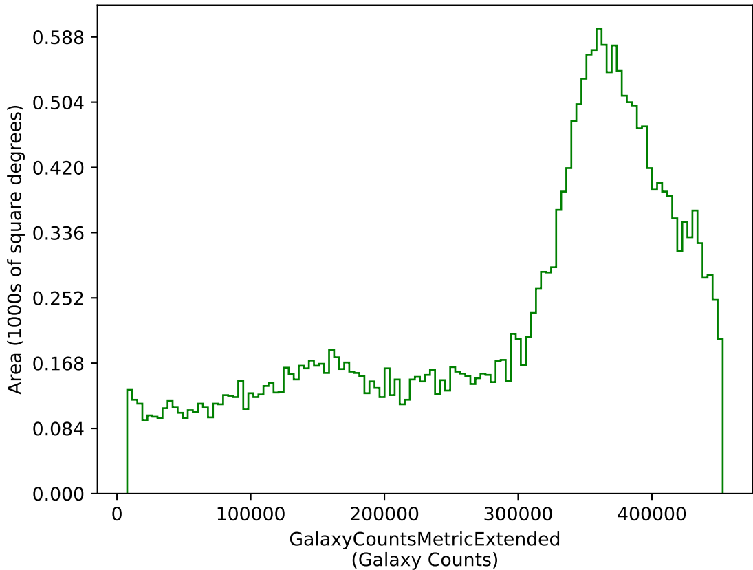
early_u_fpextra4.0_v3.4_10yrs g: GalaxyCountsMetricExtended
