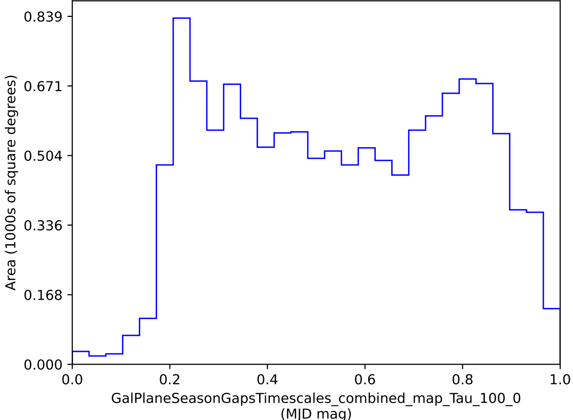
early_u_fpextra4.0_v3.4_10yrs : GalPlaneSeasonGapsTimescales_combined_map_Tau_100_0
