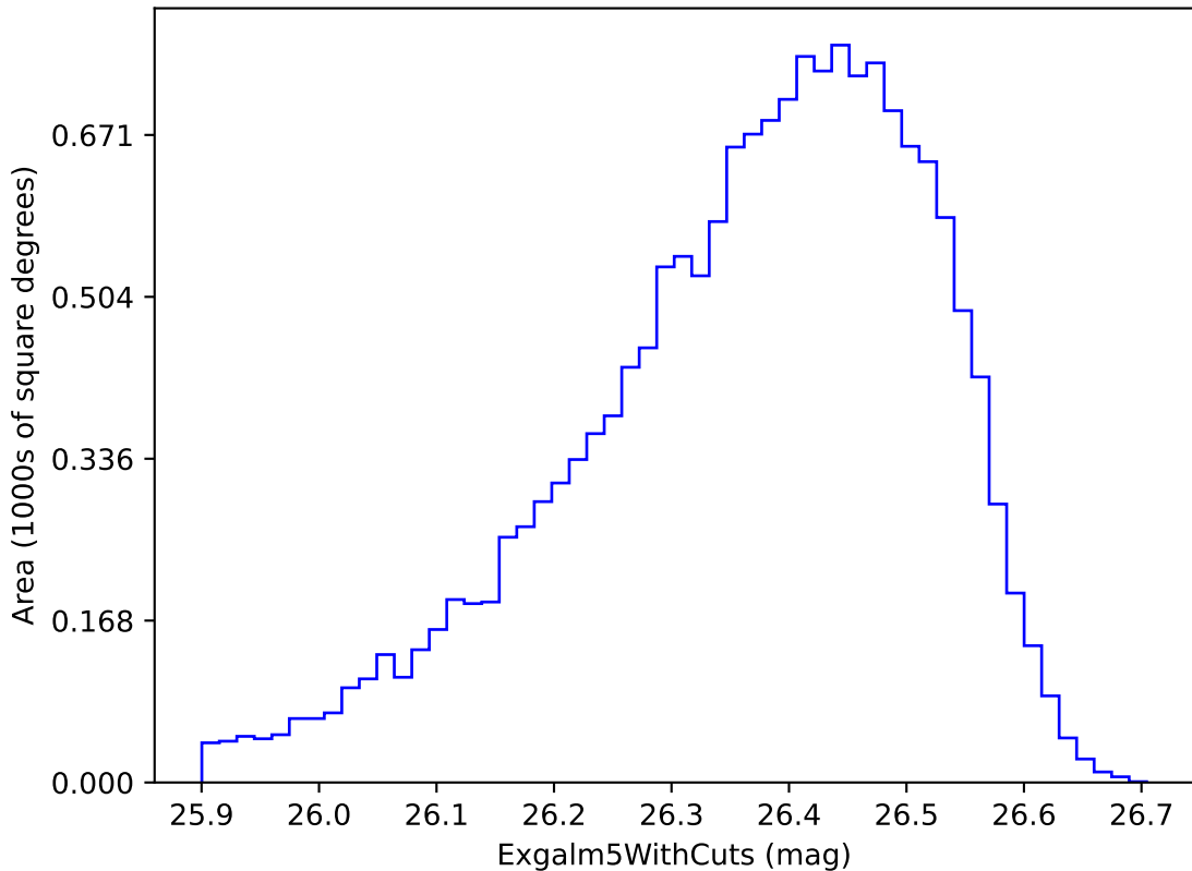
early_u_fpextra4.0_v3.4_10yrs i band non-DD year 10: ExgalM5WithCuts
