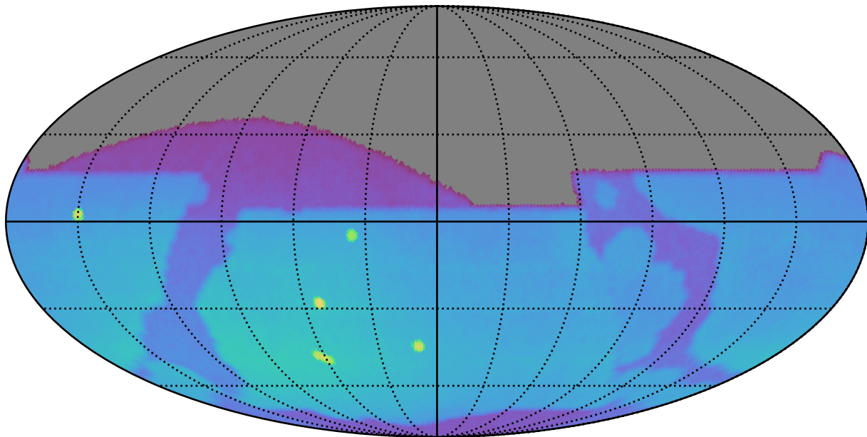
early_u_fpextra4.0_v3.4_10yrs : Brown Dwarf, L4
