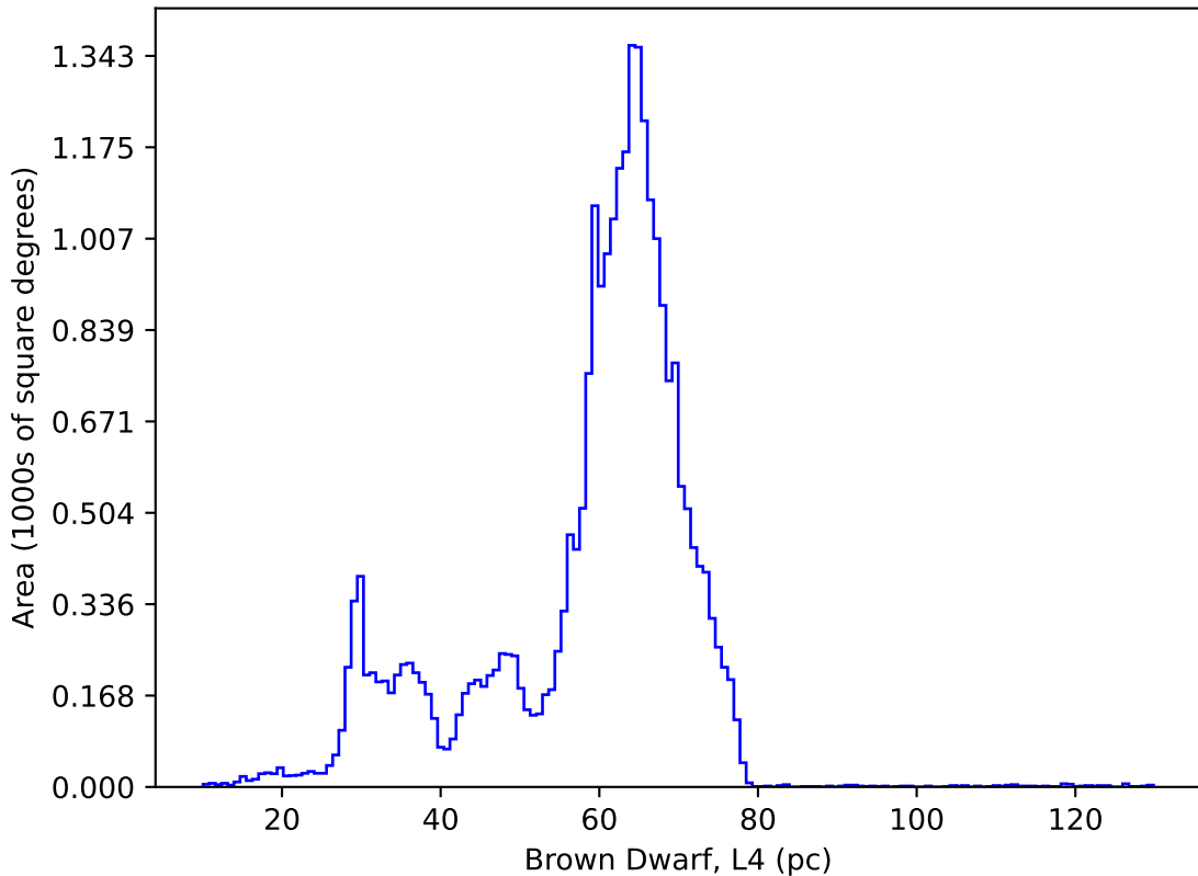
early_u_fpextra4.0_v3.4_10yrs : Brown Dwarf, L4
