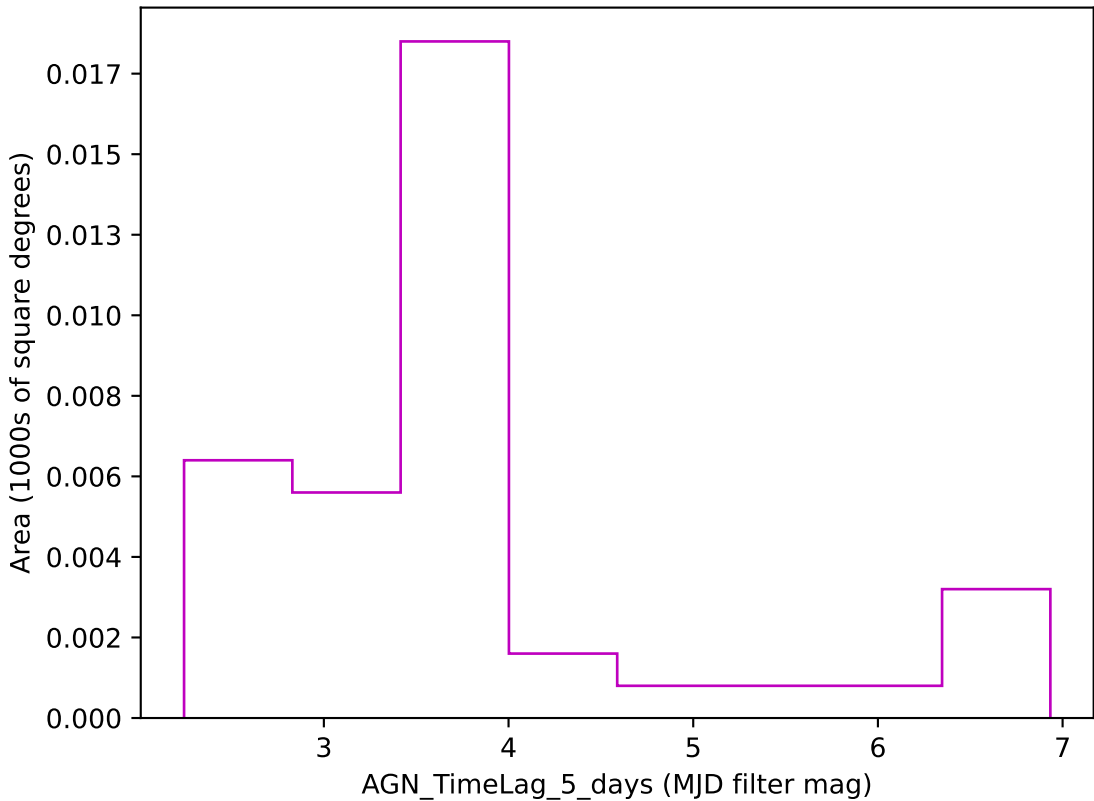
early_u_fpextra4.0_v3.4_10yrs z band: AGN_TimeLag_5_days
