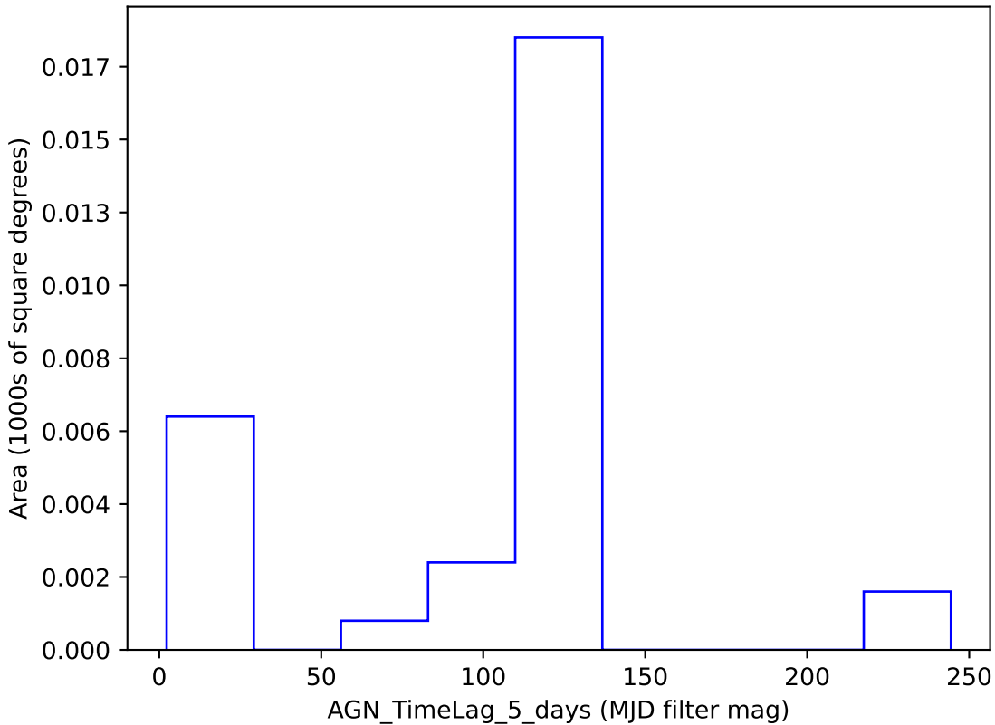
early_u_fpextra4.0_v3.4_10yrs y band: AGN_TimeLag_5_days
