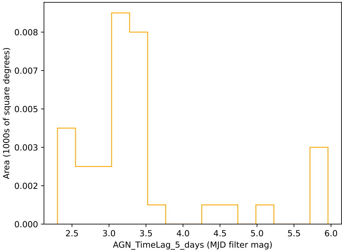
early_u_fpextra4.0_v3.4_10yrs r band: AGN_TimeLag_5_days
