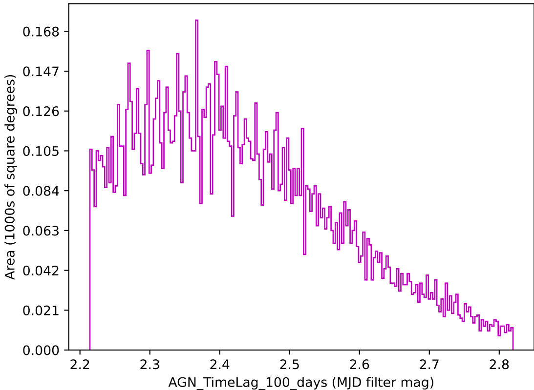
early_u_fpextra4.0_v3.4_10yrs z band: AGN_TimeLag_100_days
