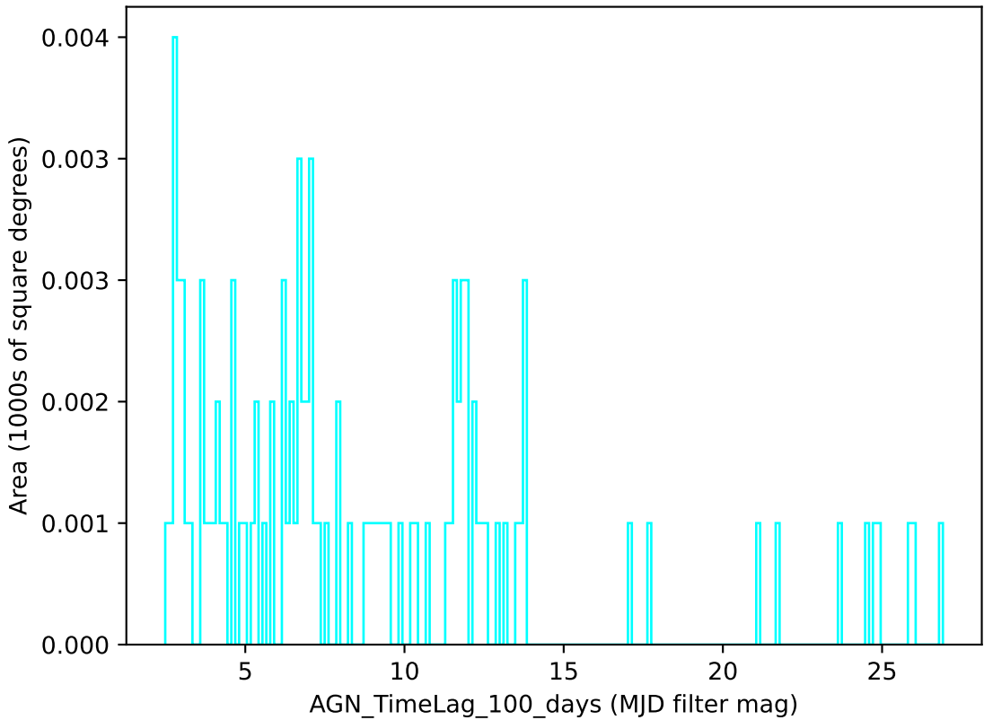
early_u_fpextra4.0_v3.4_10yrs u band: AGN_TimeLag_100_days
