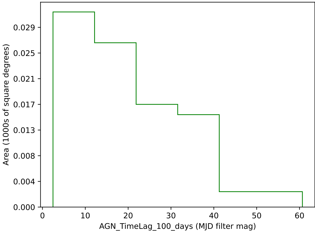
early_u_fpextra4.0_v3.4_10yrs g band: AGN_TimeLag_100_days
